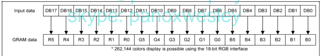
Image Data format for 16bit RGB interface (65k color)
