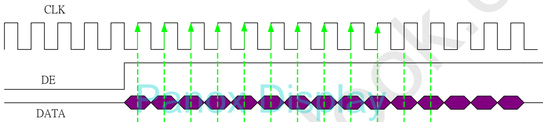
Image Data format for 18bit RGB interface (262k color)
