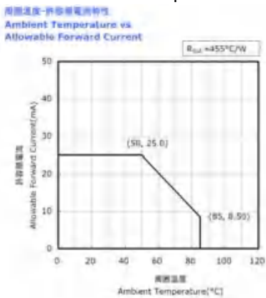
Fig.1 LED Characteristic(De-rating Curve)
